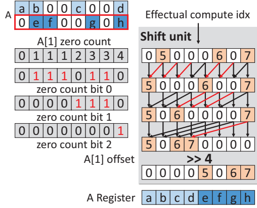
Fig. 12: Example of shift unit.
