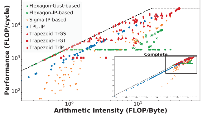
Fig. 21: Log-log roofline of all workloads.
