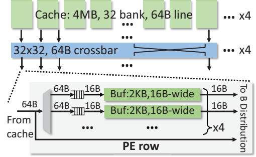
Fig. 13: Multi-level memory hierarchy.
