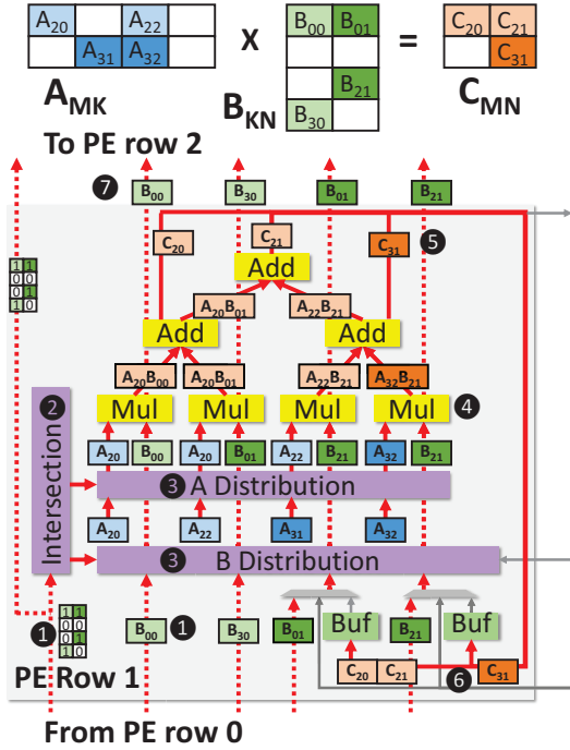
Fig. 10: Example of Trapezoid running TriP for MSxMS.
