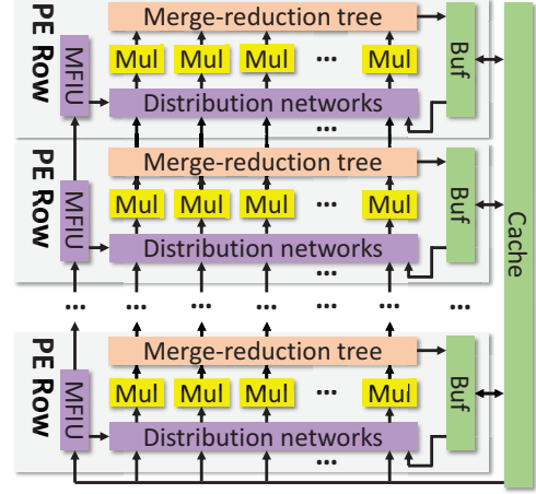
Fig. 5: Trapezoid architecture overview.
